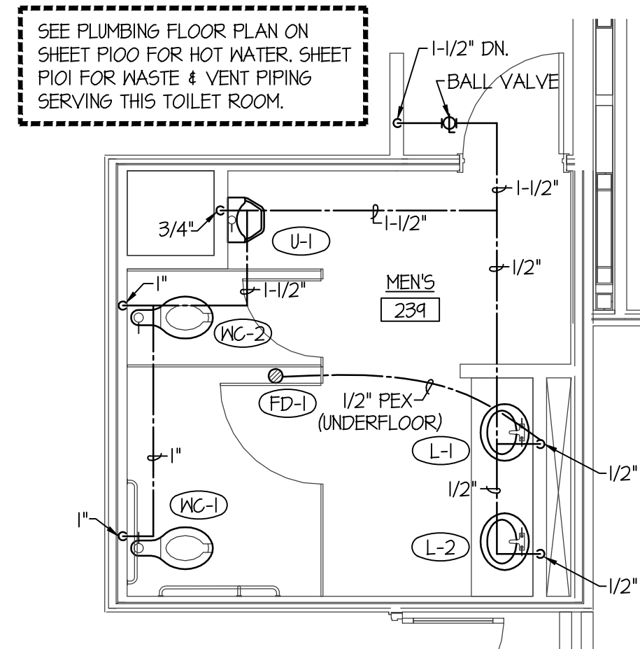
LARGE SCALE MEN'S 239 PLUMBING PLAN
