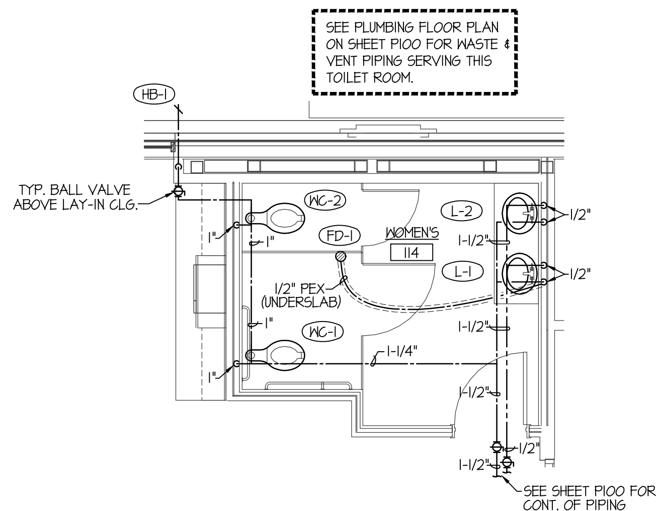
LARGE SCALE WOMEN'S 114 PLUMBING PLAN
