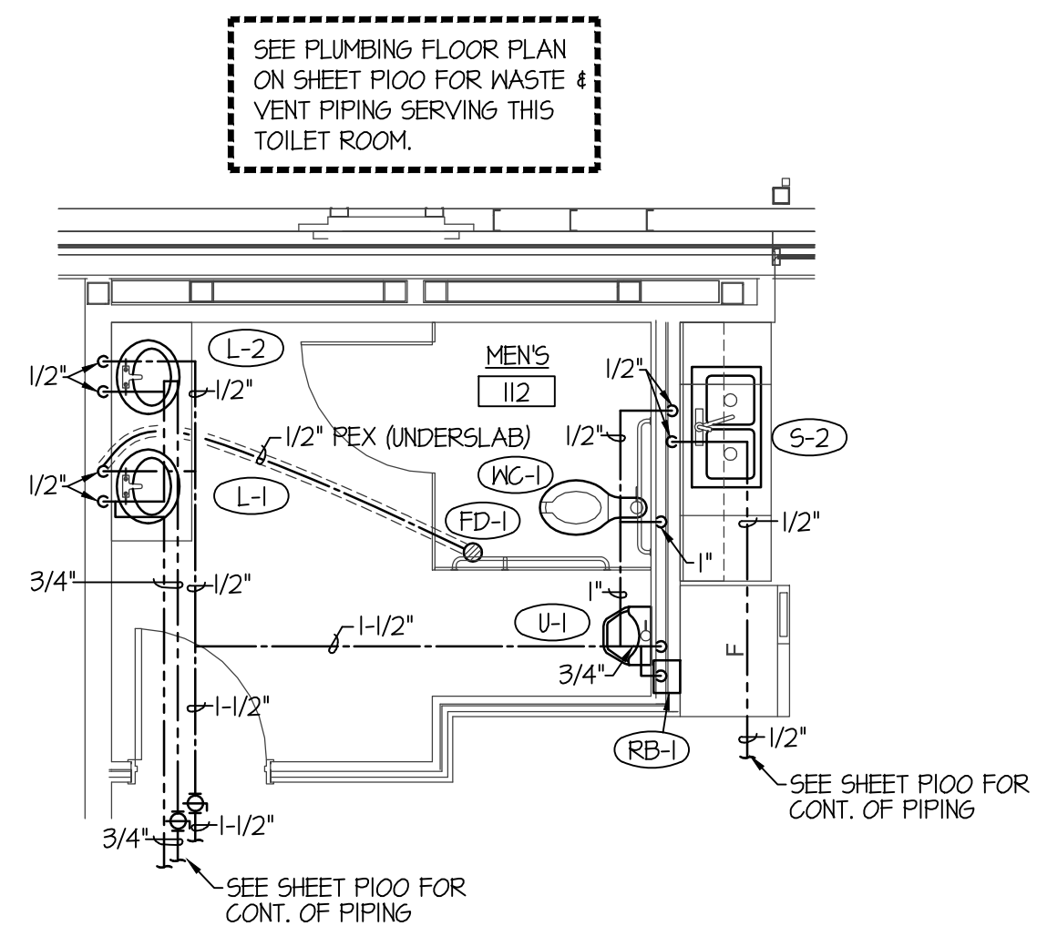
LARGE SCALE MEN'S 112 PLUMBING PLAN
