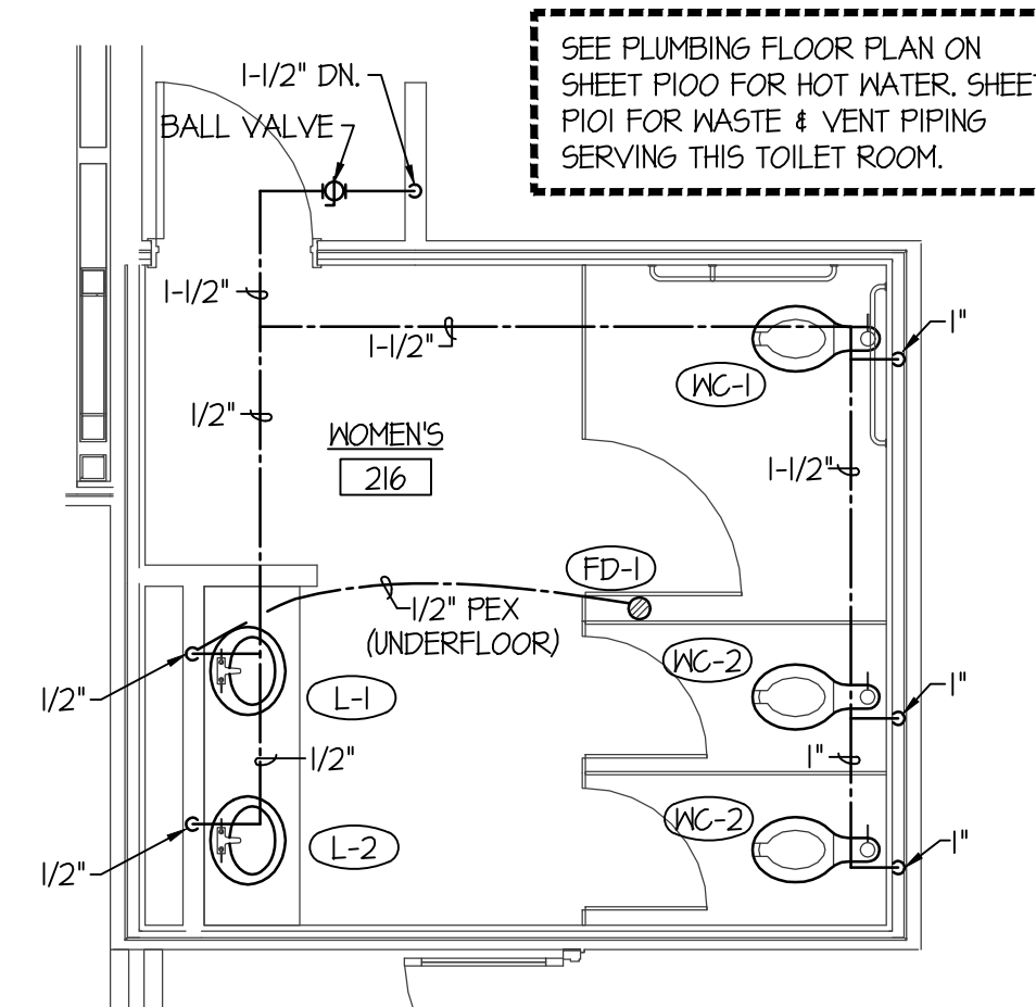
LARGE SCALE WOMEN'S 216 PLUMBING PLAN
