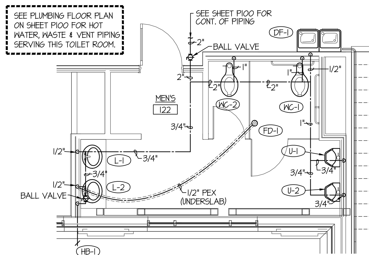
LARGE SCALE MEN'S 122 PLUMBING PLAN
