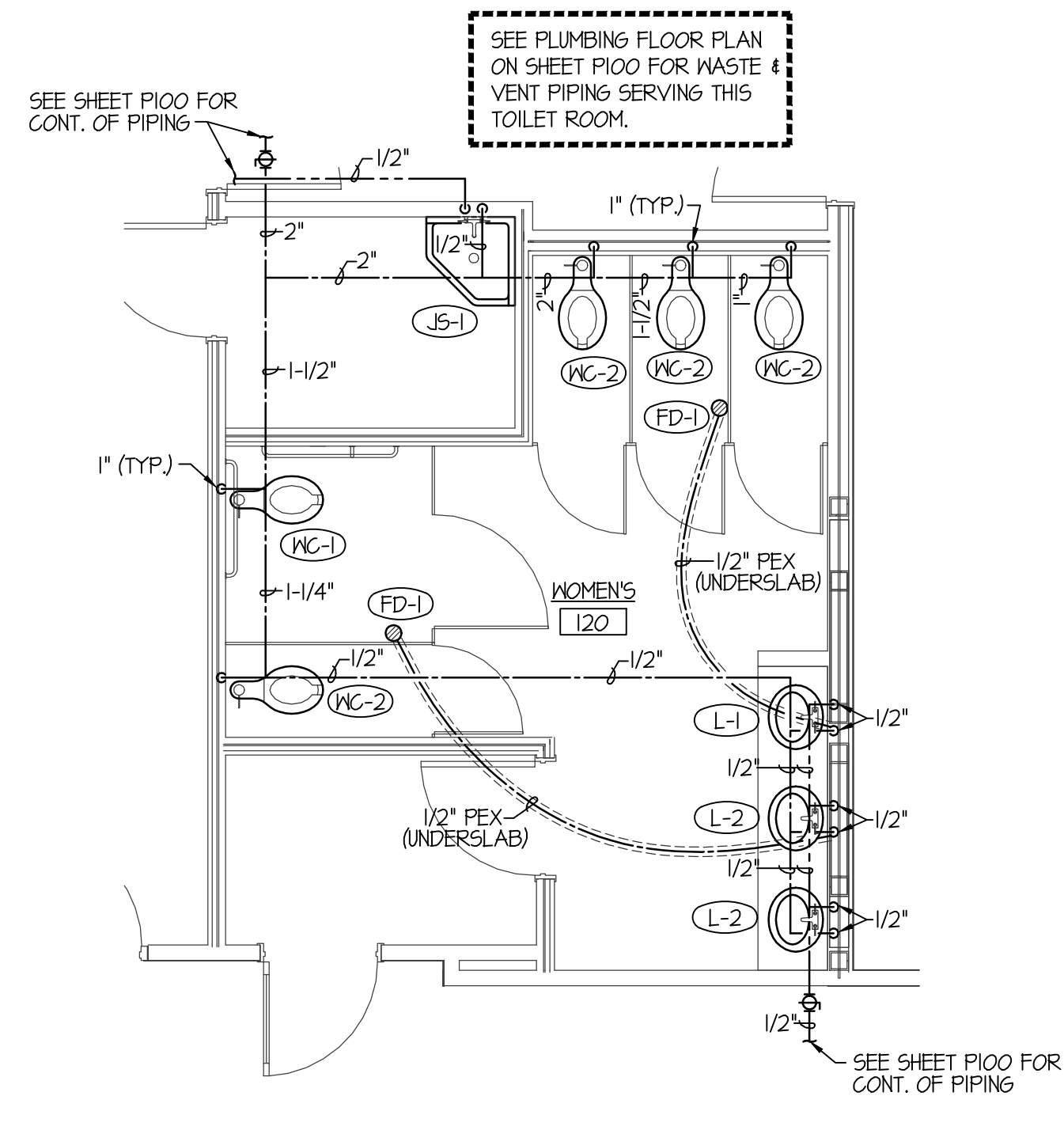
LARGE SCALE WOMEN'S 120 PLUMBING PLAN
